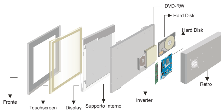
Modularized Construction
