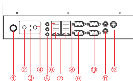
Chassis
