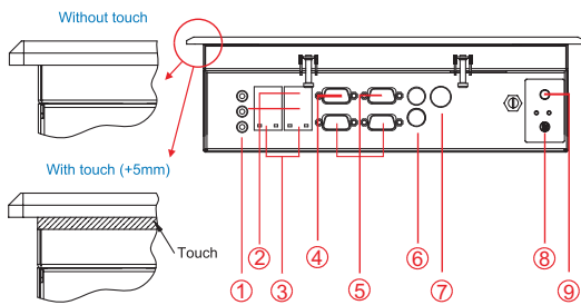
Panel Mount (5mm front bezel)
