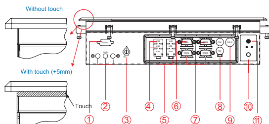
Panel Mount (5mm front bezel)
