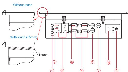
Panel Mount (5mm front bezel)
