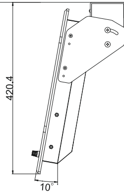
ROOF MOUNT
