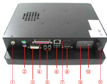
Chassis
