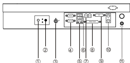
Chassis
