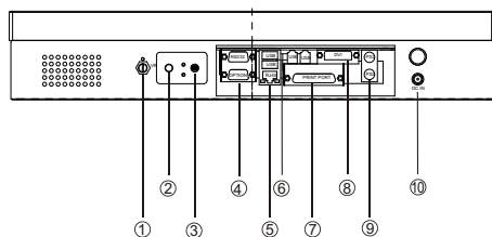
Chassis
